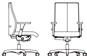
LL / LM / LF / LG / LGM50 BW 18" SW 18.5" BH 19.5-22" SH 17-20.5" SD 17.5"
