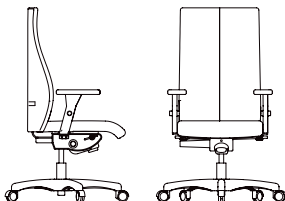
LL / LM / LF / LG / LGM90 BW 18" SW 18.5" BH 23.5-26" SH 17-20.5" SD 17.5"
