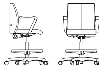
LL / LF / LM80 BW 18" SW 18.5" BH 16.5" SH 23-33" SD 17.5"
