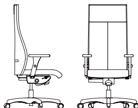
LL / LM / LG / LGM92 BW 18" SW 18.5" BH 28.5-31" SH 17-20.5" SD 17.5"
