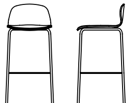
KC26 BW 16" SW 17" BH 8" SH 30" SD 18"
