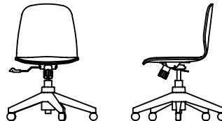
KO41 BW 16" SW 17" BH 15" SH 17.75" SD 18"
