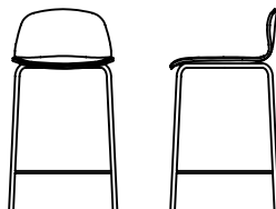
KC36 BW 16" SW 17" BH 8" SH 26" SD 18"
