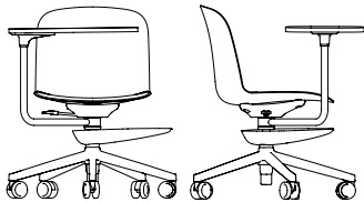
RP40 SW 17.5" BH 14.5" SH 17 - 21.5" SD 16.25" OW 25.4"
