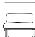
OVE31 BW 38" SW 47.5" BH 15" SH 17.5" SD 26.25"
