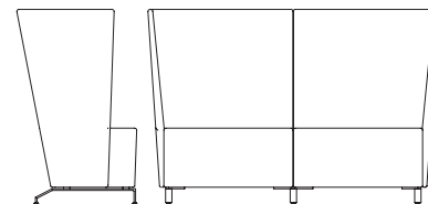
VW42PDG H 46" W 24" L 64"
