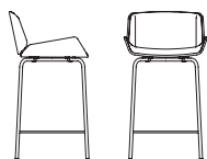
MAR35 BW 18.5" SW 19.5" BH 13" SH 26" SD 16.5"
