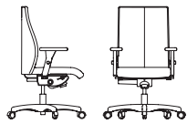
LL/ LR/ LM/ LF/ LG/ LGM 50 BW 18" SW 18.5" BH 19.5-22" SH 17-20.5" SD 17.5"
