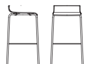
PC 25/ 26/ 27 BW 16.25" SW 16.25" BH 4.5" SH 30" SD 15"
