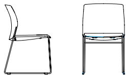
LE72 / LE76 / LP72 / LP76 LD 18" LS 18" HD 15.75" HS 18" PS 18.5"
