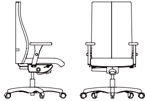
LM / LG / LGM90 LD 18" LS 18,5" HD 23,5-26" HS 17-20,5" PS 17,5"
