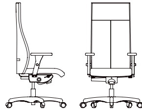
LM / LG / LGM92 LD 18" LS 18,5" HD 28,5-31" HS 17-20,5" PS 17,5"
